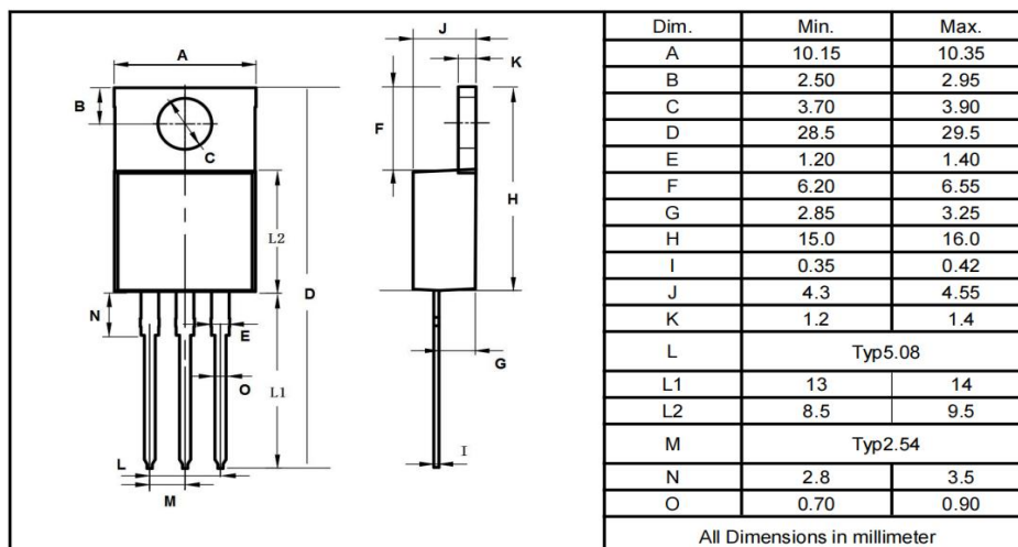
TO-220AB
